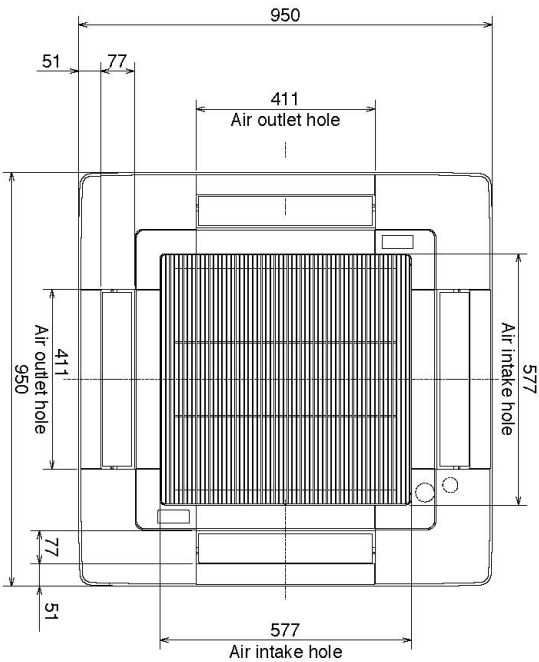
Lower View >
