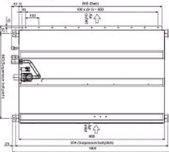
Upper View >
