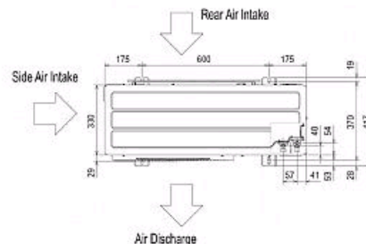
Upper View >
