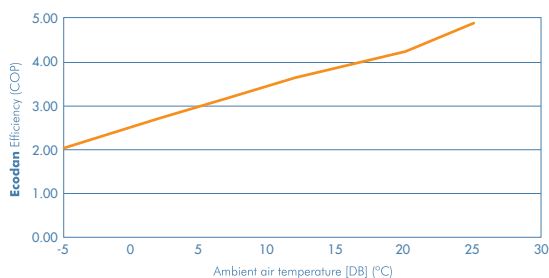
BRE test data - hot water cylinder heat up
