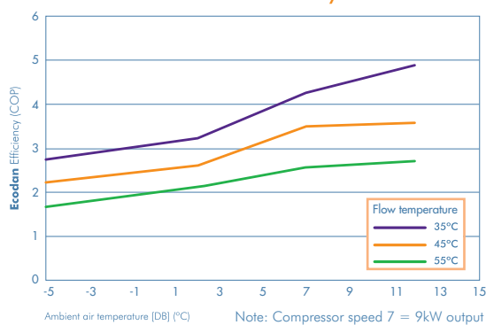
BRE test data - Ecodan efficiency test
